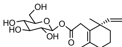
fruit fly (M sex phe.)
