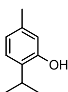
scentless plant bug (gland secretion)
