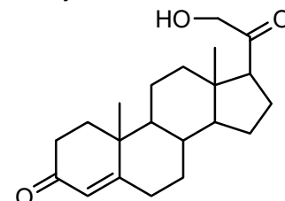
water beetle, aquatic bug (allomone)
