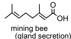
geranolic acid
