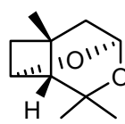
lineatin
