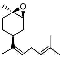
\alpha -bisabolene epoxide
