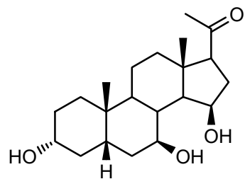
burying beetle (allomone)
