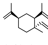
\beta -elemene
