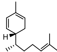
zingiberene
