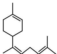
\alpha -bisabolene
