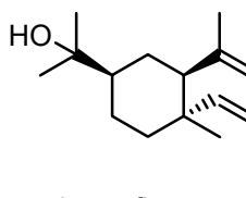
\alpha -elemol
