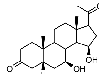
burying beetle (allomone)
