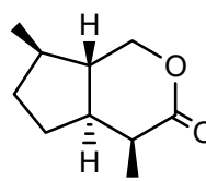
parasitoid wasp (allomone)
