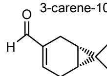
3-carene-10-ol
