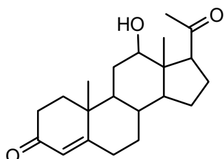
6-dehydropregesterone
