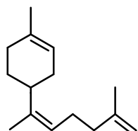
\alpha_2 -bisabolene
