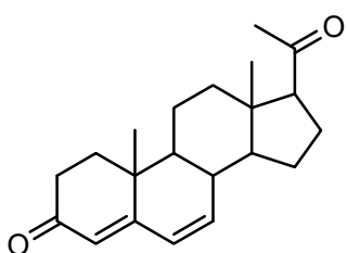
6-dehydropregesterone
