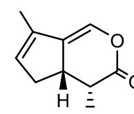
leaf beetle (allomone)
