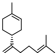
\beta -bisabolene
