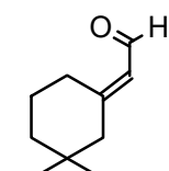
grandlure III
