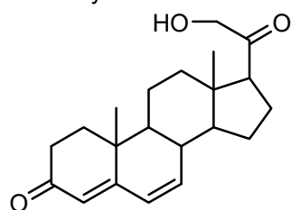
6-dehydrocortexone
