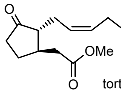
methyl jasmonate
