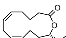
cucujolide X
