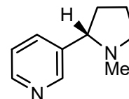
harvestman (allomone ?)
