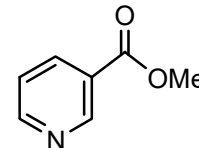
methyl nicotinate
