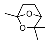
ant, bee (gland secretion)
